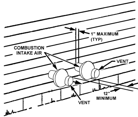
Figure 31: CONCENTRIC VENT TERMINATIONS FOR HORIZONTAL DIRECT VENTING
