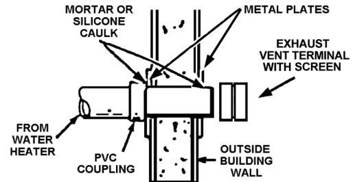
EXHAUST VENT TERMINAL - ALL MODELS
