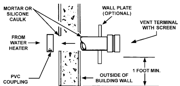
Figure 13: VENT TERMINATION
